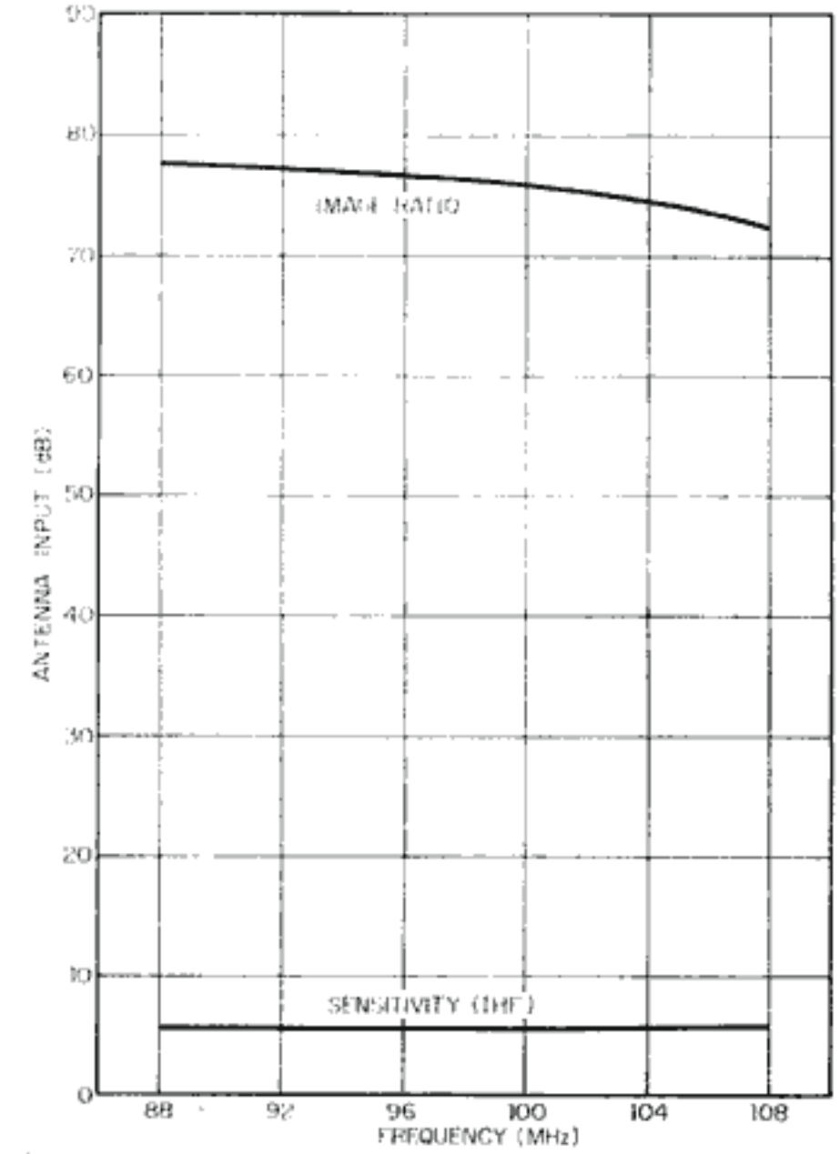
FM SENSITIVITY & IMAGE RATIO
