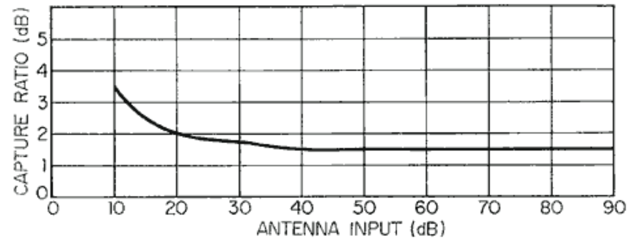
CAPTURE RATIO (IHF)
