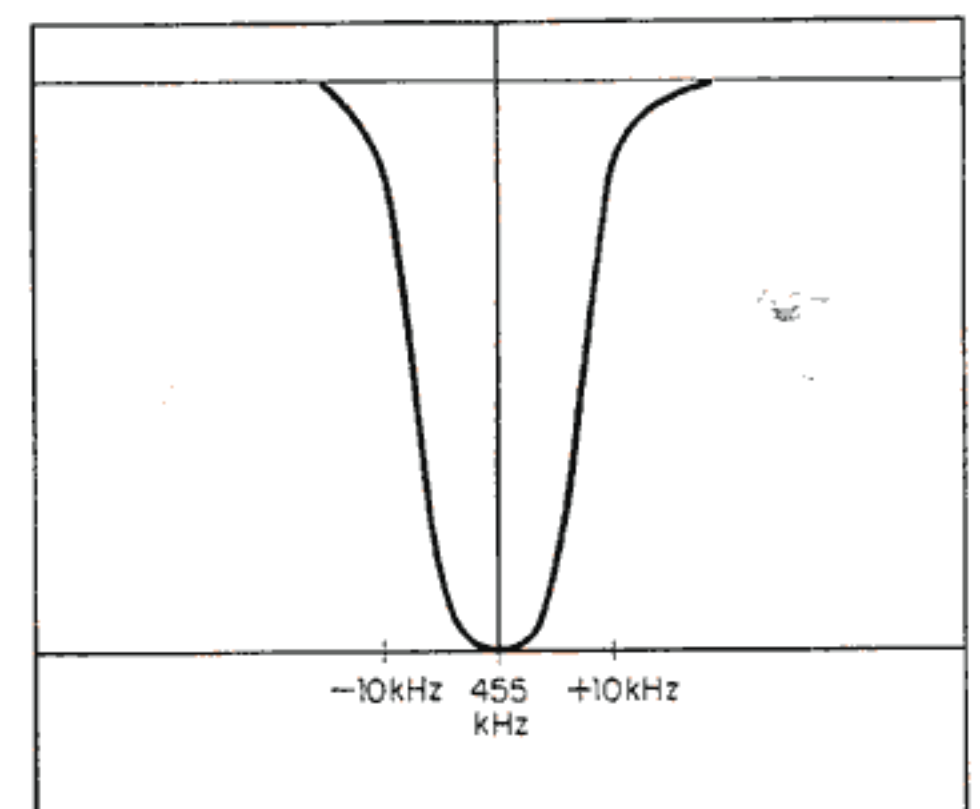
AM IF CHARACTERISTIC
