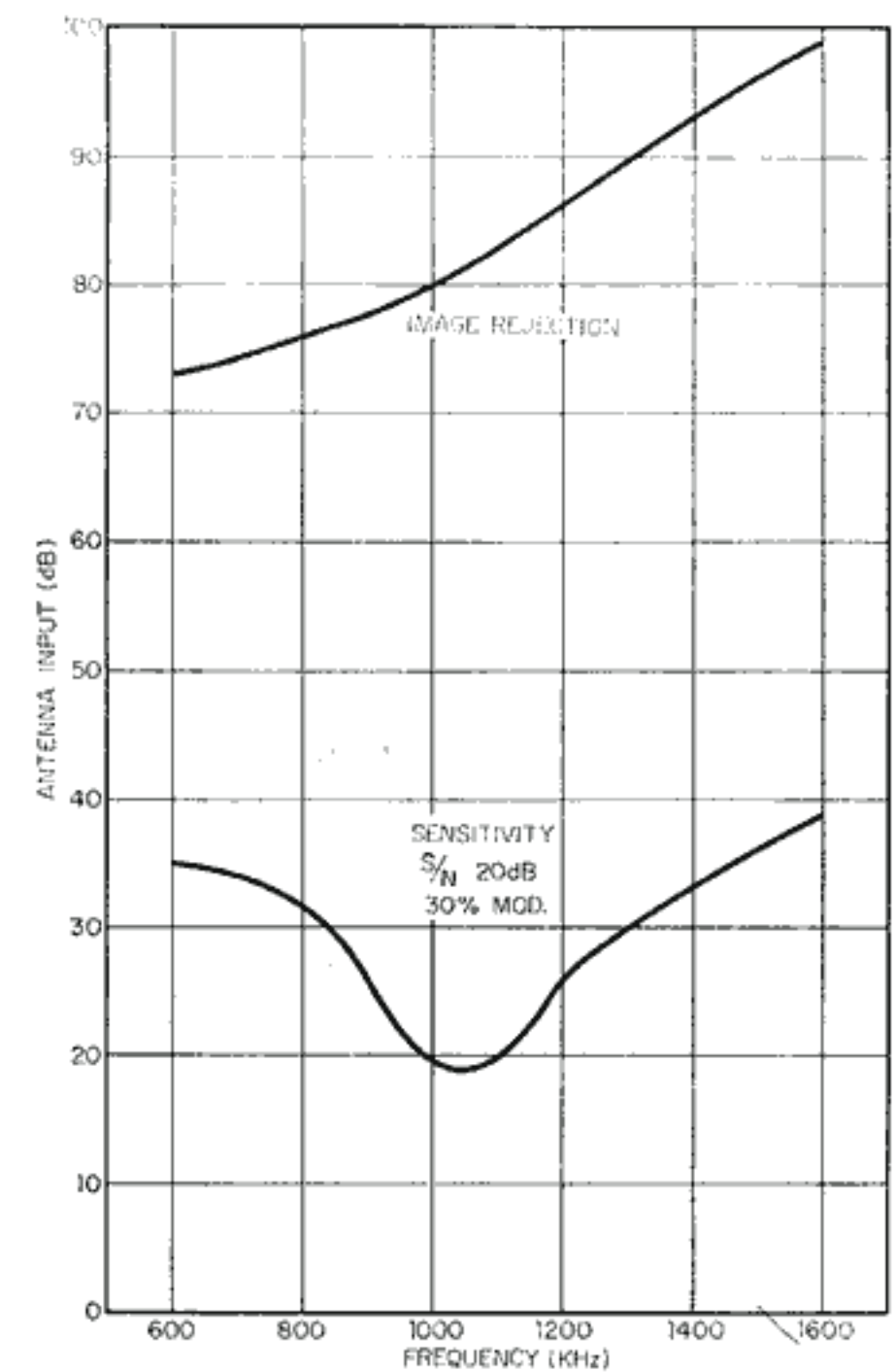
AM SENSITIVITY & IMAGE REJECTION
