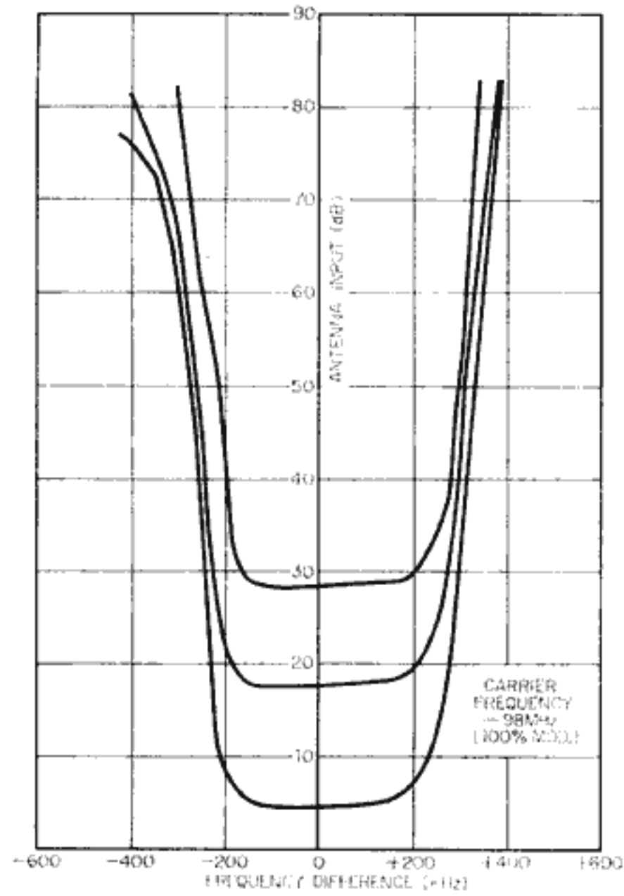
FM SELECTIVITY
